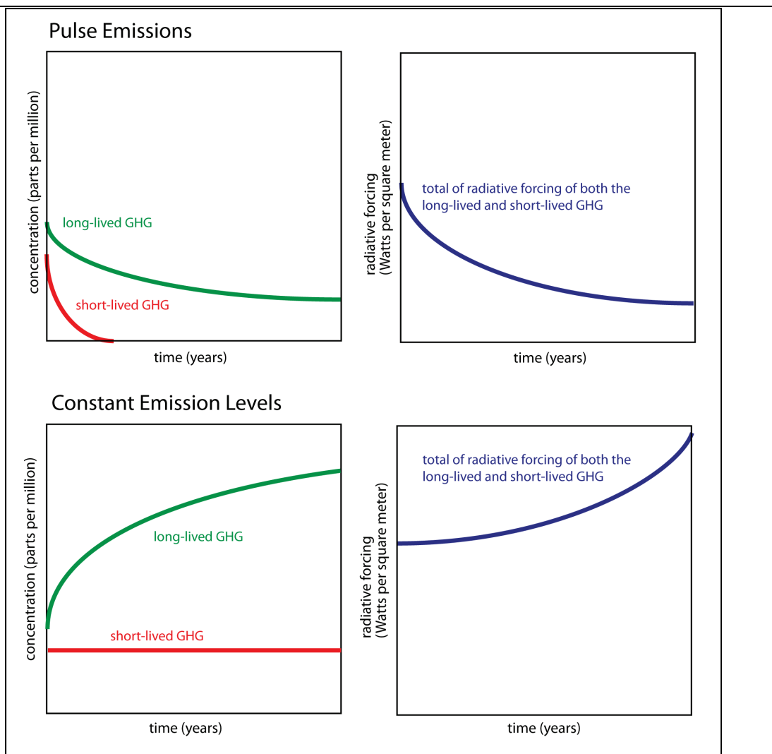
Figure 5: Atmospheric Concentration and Radiative Forcing Over Time for a Pulse Emission (top) and Constant Emission Levels (bottom).
