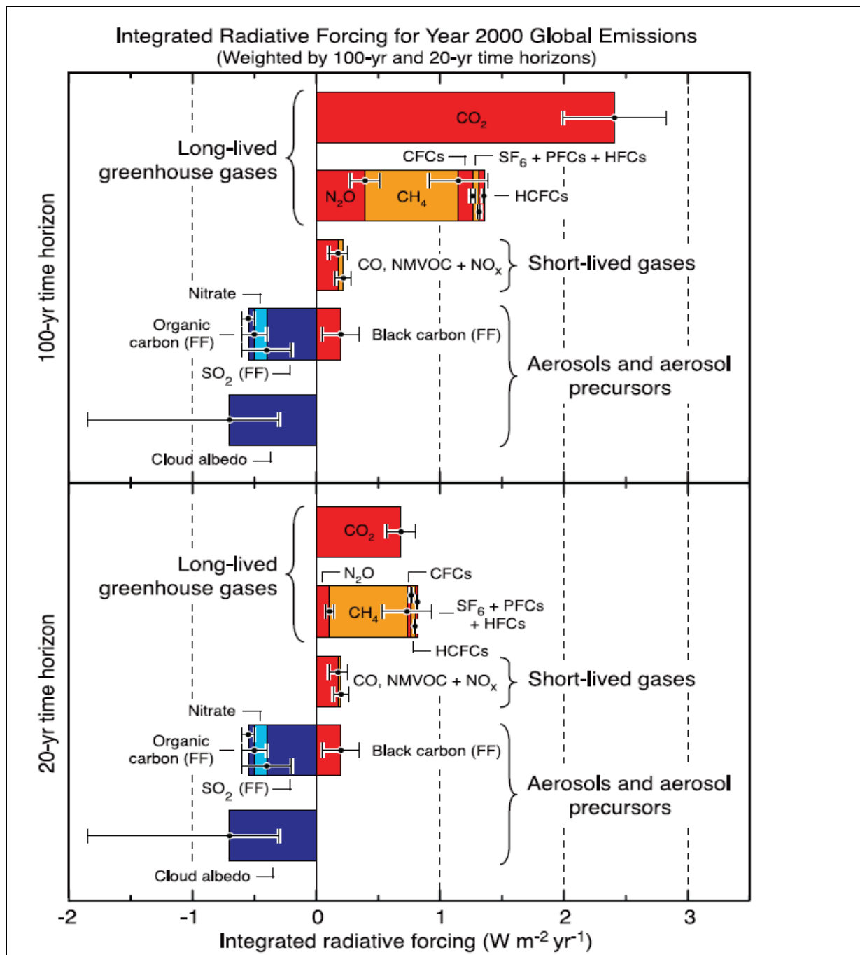
Figure 4: Integrated RF of All Anthropogenic GHGs Emitted in the Year 2000 over Two Different Time Horizons.
