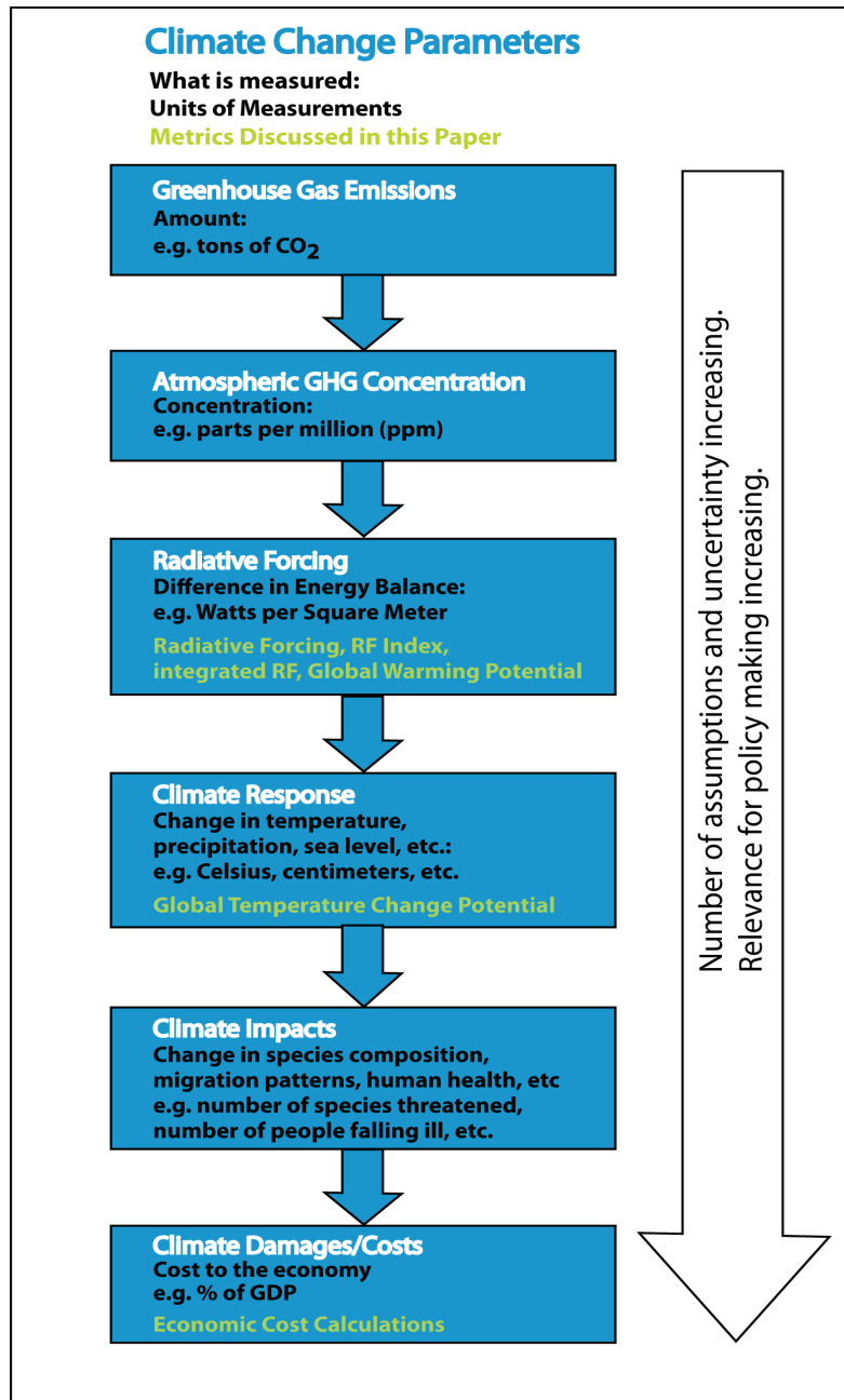
Figure 9: Climate Change Parameters and Their Associated Metrics.
