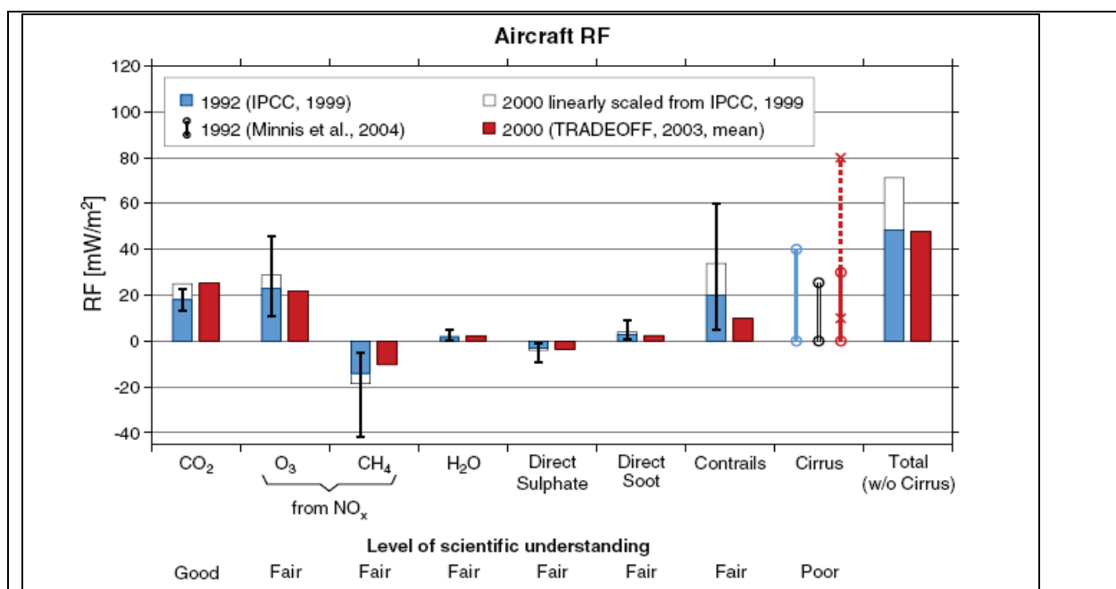
Figure 2: Radiative Forcing of Aircraft Emissions in 1992 and 2000 (emissions from 1940 to 2000) (Source: Sausen et al., 2005)
