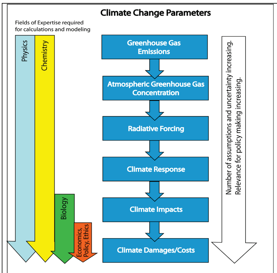
Figure 1: Measuring Climate Impacts
